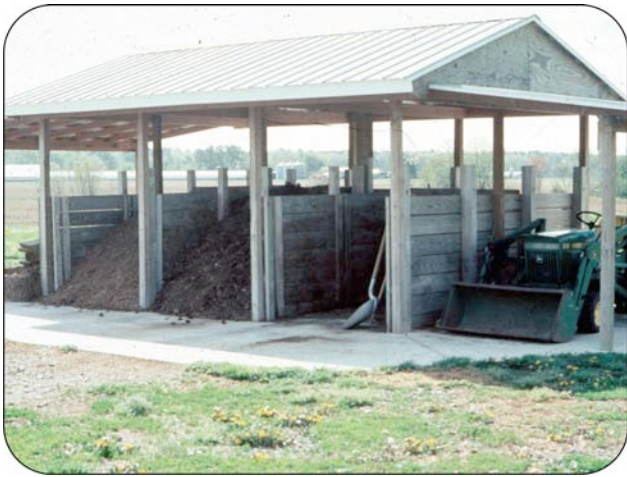
Figure 3. Three-bin composting system.
