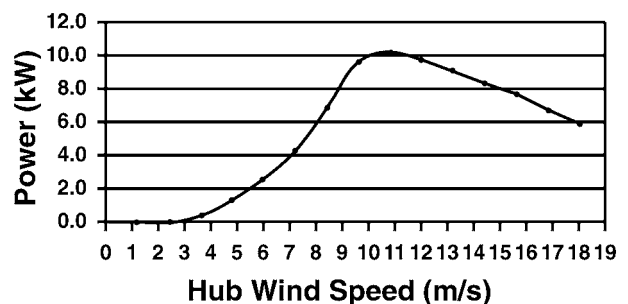
FIGURE 10. Examples of a power curve for a small wind turbine rated at 10 kW. (Source: Atlantic Orient Corporation)
