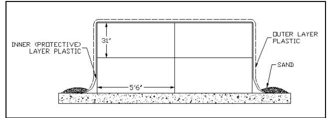
FIGURE 9. Big square bale stack face (stacks should be 5–10 bales long)
