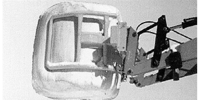
FIGURE 3. Individually wrapped round bale and handling loader attachment
